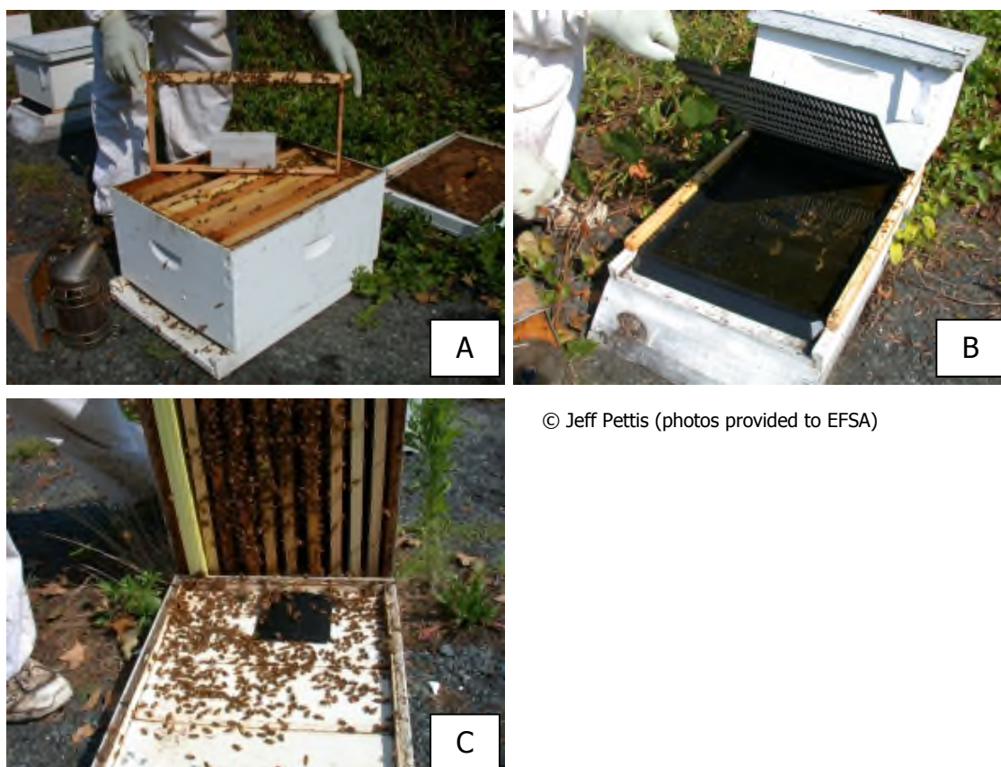
Figure 27: (A) Hood trap, (B) West trap and (C) CheckMite+ trap
